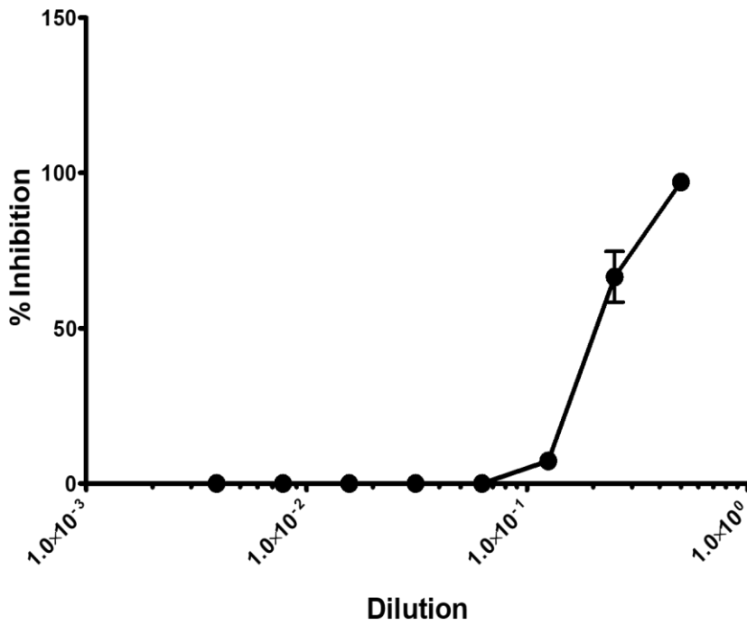
Figure 1: IM/Q610/419-01A-18 inhibition of SARS-CoV-2. The virus was incubated with IM/Q610/419-01A-18 before infection of 293T-ACE cells. After 72 hours incubation the inhibition of infection was determined by measuring luminescence. Data shown represent the results of three independent experiments, and bars represent the means \pm standard deviation
